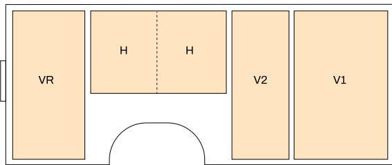
CURBSIDE VIEW (ROADSIDE SIMILAR)
